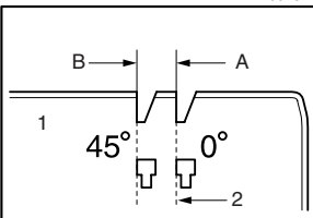
1. Base plate 2. Cutting line
