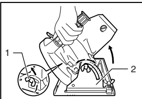
1. Wing nut 2. Bevel scale plate
