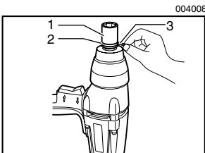
1. Socket 2. O-ring 3. Pin
